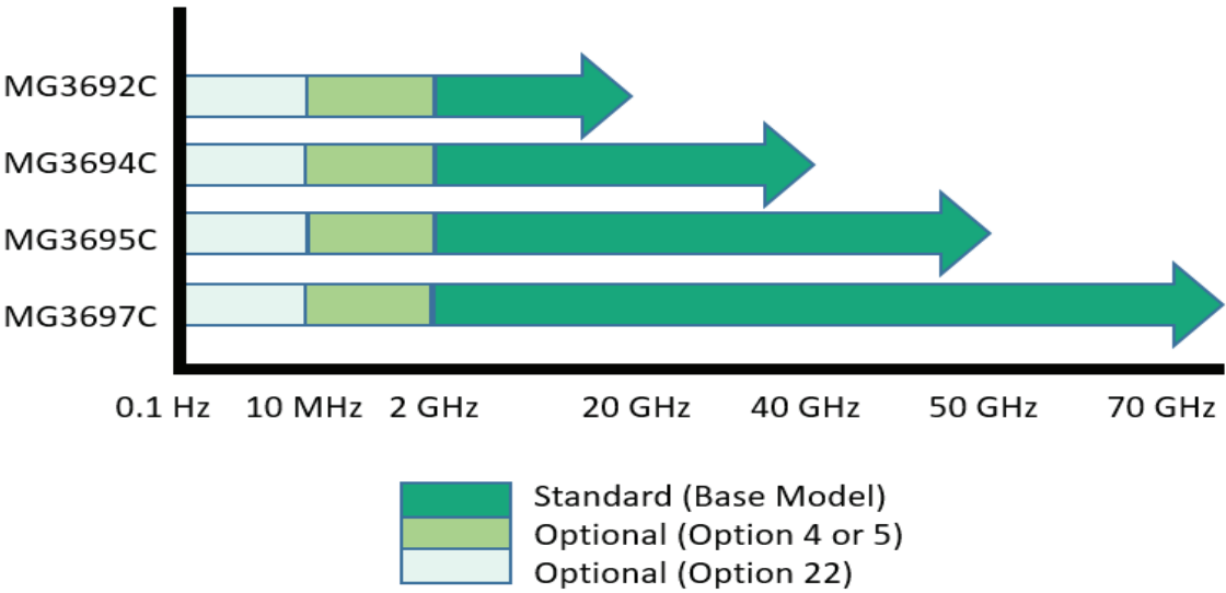
Figure 1. MG3690C Series of Broadband Signal Generators
