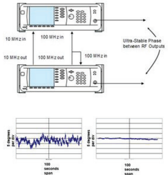
Figure 4. Precision Clock Source Setup
